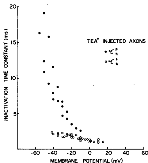
FIGURE 2 Inactivation time constants during step depolarizations (open symbols) and as derived from prepulse experiments (solid symbols) as a function of membrane potential. See Goldman and Schaaf (1973) and Schaaf and Davis (1975) for details of computational procedures.
